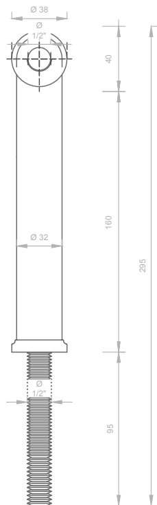
02 FRONT ELEVATION - UPSTANDS 1:2
