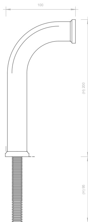
03 LEFT ELEVATION - UPSTANDS 1:2
