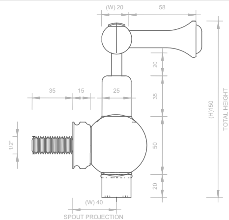
05 SIDE ELEVATION - GLOBE TAPS - HOT 1 : 2
