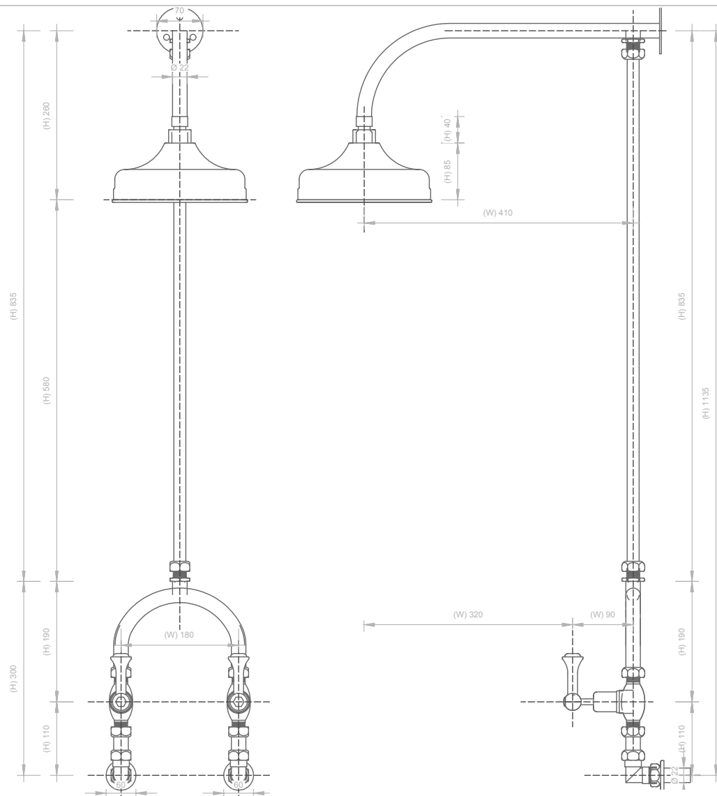
01 FRONT ELEVATION - FARMHOUSE SHOWER 1 : 5
