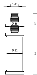
04 EXTENSION PIECE 75MM 1 : 2
