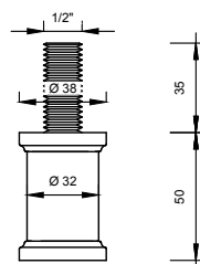
03 EXTENSION PIECE 50MM 1 : 2
