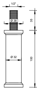
02 ELEVATION - EXTENSION PIECE 1 : 2
