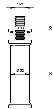
05 EXTENSION PIECE 100MM 1 : 2
