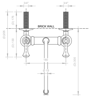
02 FRONT ELEVATION - BRIDGE SINK MIXER - WALL MOUNTED 1 : 5
