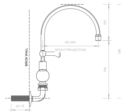
03 LEFT ELEVATION - BRIDGE SINK MIXER - WALL MOUNTED 1 : 5
