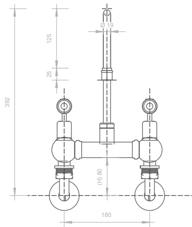
02 FRONT ELEVATION - BRIDGE SINK MIXER - WALL MOUNTED 1 : 5
