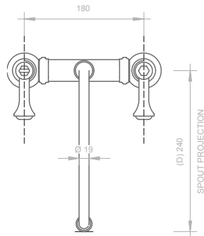
01 PLAN - BRIDGE SINK MIXER - DECK MOUNTED 1 : 5
