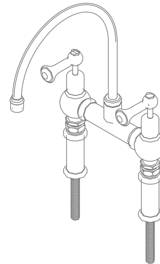
03 LEFT ELEVATION - BRIDGE SINK MIXER - DECK MOUNTED 1 : 5
