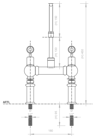
02 FRONT ELEVATION - BRIDGE SINK MIXER - DECK MOUNTED 1 : 5
