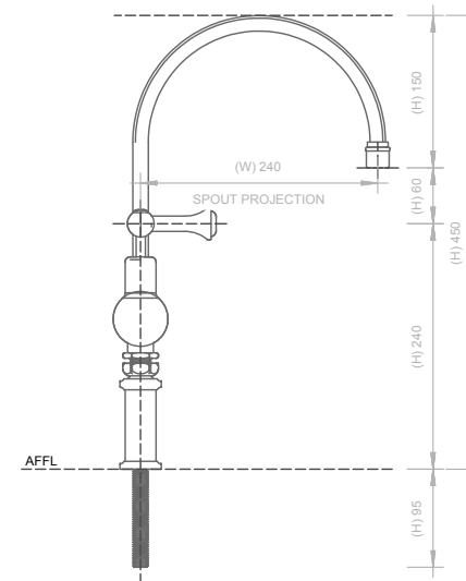
03 LEFT ELEVATION - BRIDGE SINK MIXER - DECK MOUNTED 1 : 5
