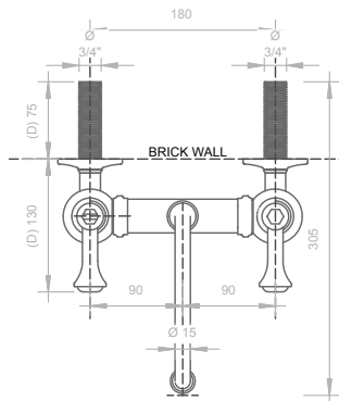
01 PLAN - BRIDGE BASIN MIXER WALL MOUNTED 1 : 5
