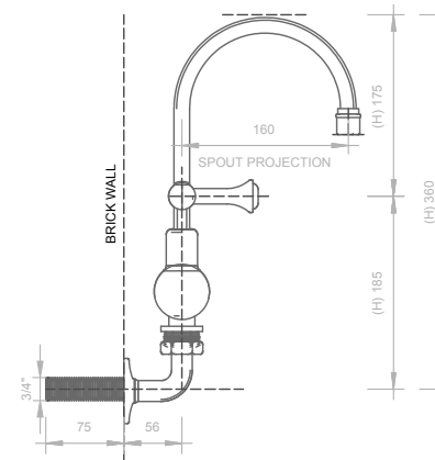
03 LEFT ELEVATION - BRIDGE BASIN MIXER WALL MOUNTED 1 : 5
