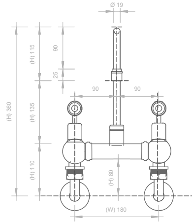
02 FRONT ELEVATION - BRIDGE BASIN MIXER WALL MOUNTED 1 : 5
