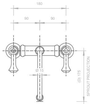
01 PLAN - BRIDGE BASIN MIXER DECK MOUNTED 1 : 5
