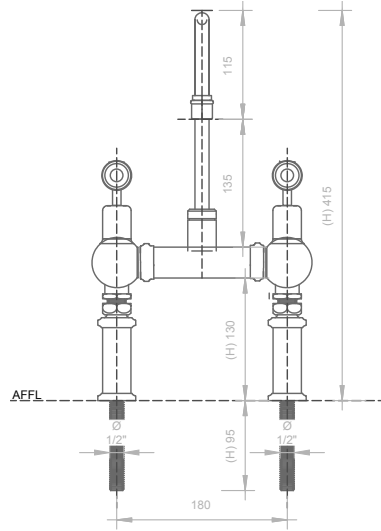
02 FRONT ELEVATION - BRIDGE BASIN MIXER DECK MOUNTED 1 : 5
