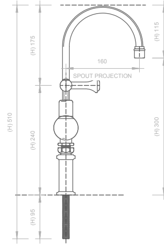
03 LEFT ELEVATION - BRIDGE BASIN MIXER DECK MOUNTED 1 : 5
