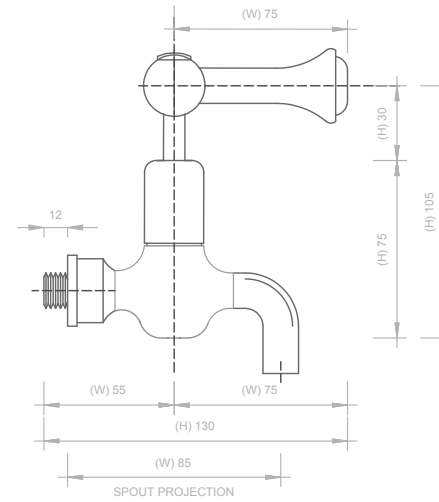
03 LEFT ELEVATION - BIB TAPS 1 : 2
