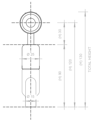
02 FRONT ELEVATION - BIB TAPS 1 : 2
