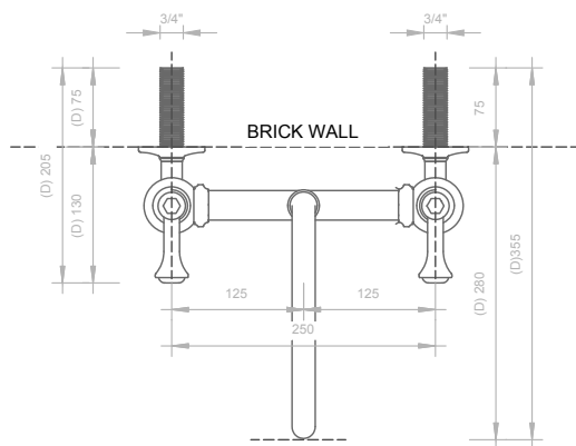
01 PLAN - BATH MIXER - WALL MOUNTED 1 : 5
