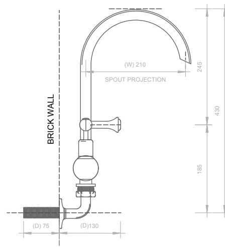
03 LEFT ELEVATION - BATH MIXER - WALL MOUNTED 1 : 5
