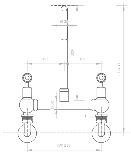
02 FRONT ELEVATION - BATH MIXER - WALL MOUNTED 1 : 5
