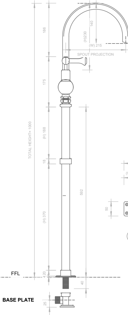
02 LEFT ELEVATION - BATH MIXER - FLOOR MOUNTED 1:5
