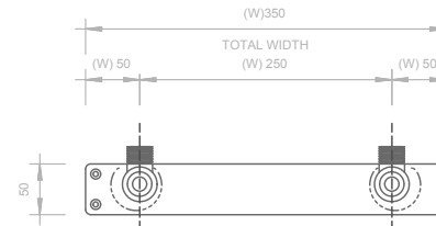
04 PLAN - BASEPLATE 1:5
