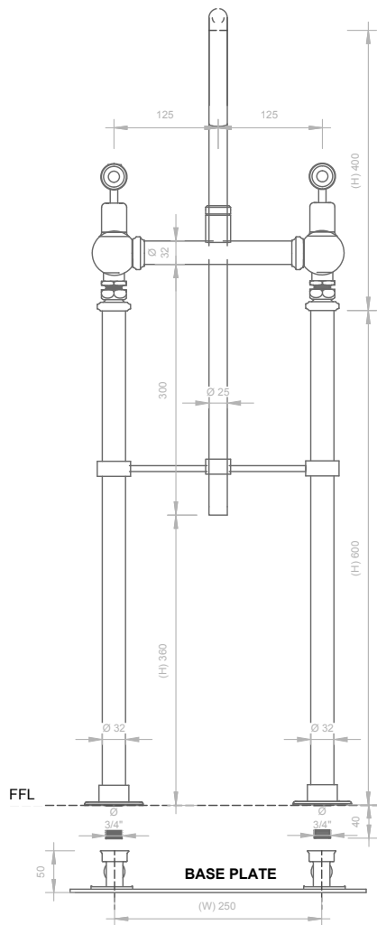
01 FRONT ELEVATION - BATH MIXER - FLOOR MOUNTED 1:5
