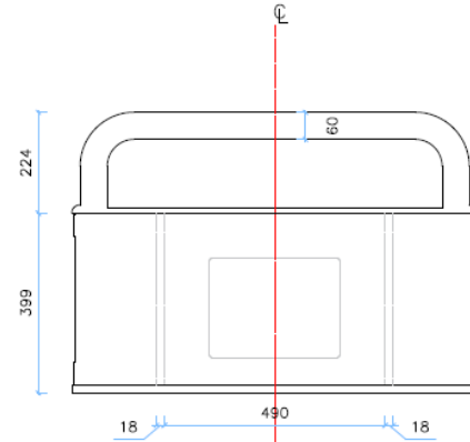
Back Elevation
