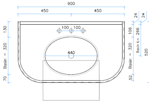
Plan - Top
