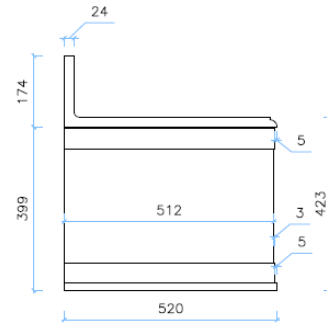
Side Elevation
