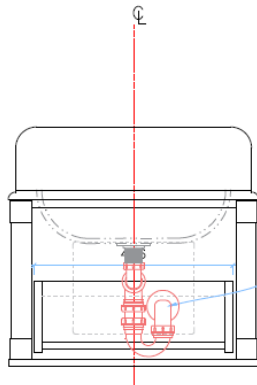
Front Elevation - Internal
