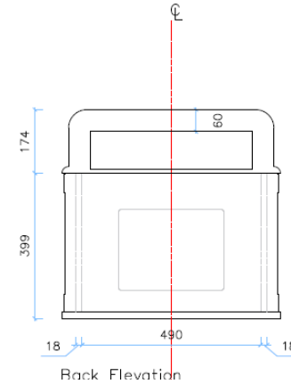
Back Elevation
