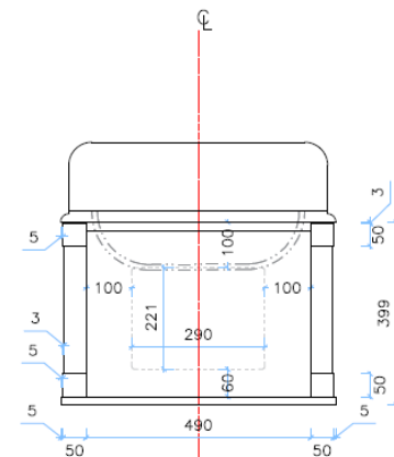
Front Elevation - Internal cutout
